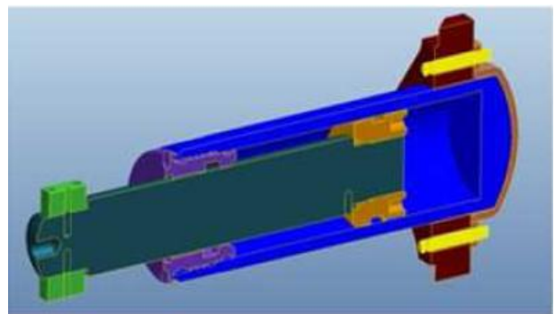
Fig. 2: A sectional view of Hydraulic Cylinder Pro Engineer Model.
