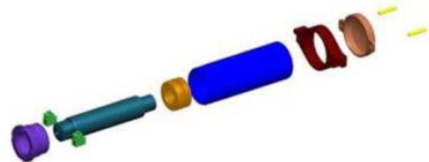
Fig. 3: An inline for assembly view of the Hydraulic Cylinder Pro Engineer Model.
